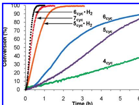
Figure 4. REMP of COE using catalysts 4_{\text{cyc}} (green), 5_{\text{cyc}} (purple), 5_{\text{cyc}}\cdot\text{H}_2 (orange), 6_{\text{cyc}} (blue), 6_{\text{cyc}}\cdot\text{H}_2 (black), and 7_{\text{cyc}} (red). Conditions: \text{CD}_2\text{Cl}_2 , 40^\circ\text{C} , [\text{M}/\text{C}]_0 = 1000:1 , [\text{M}]_0 = 0.5 M. Conversion determined by ^1\text{H} NMR spectroscopy.
