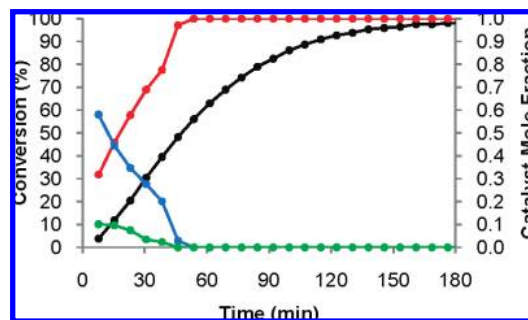
Figure 6. Left axis: Conversion of COE to PCOE using 5_{\text{acyc}} (black). Right axis: Mole fraction of 5_{\text{cyc}} (red), 5_{\text{acyc}} (blue), and A (green). Conditions: \text{CD}_2\text{Cl}_2 , 40 °C, [\text{COE}/5_{\text{acyc}}]_0 = 250 :1, [\text{COE}]_0 = 0.5 M. Conversion determined by ^1\text{H} NMR spectroscopy.
