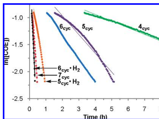
Figure 5. Log plots for REMP of COE using catalysts 4_{\text{cyc}} (green), 5_{\text{cyc}} (purple), 5_{\text{cyc}}\cdot\text{H}_2 (orange), 6_{\text{cyc}} (blue), 6_{\text{cyc}}\cdot\text{H}_2 (black), and 7_{\text{cyc}} (red). Linear least-squares fitting gave R^2 values of the following: 4_{\text{cyc}} , 0.997; 5_{\text{cyc}} , 0.969; 5_{\text{cyc}}\cdot\text{H}_2 , 0.991; 6_{\text{cyc}} , 0.998; 6_{\text{cyc}}\cdot\text{H}_2 , 0.990; and 7_{\text{cyc}} , 0.991. Conditions: \text{CD}_2\text{Cl}_2 , 40^\circ\text{C} , [\text{M}/\text{C}]_0 = 1000:1 , [\text{M}]_0 = 0.5 M. Data recorded using ^1\text{H} NMR spectroscopy.
