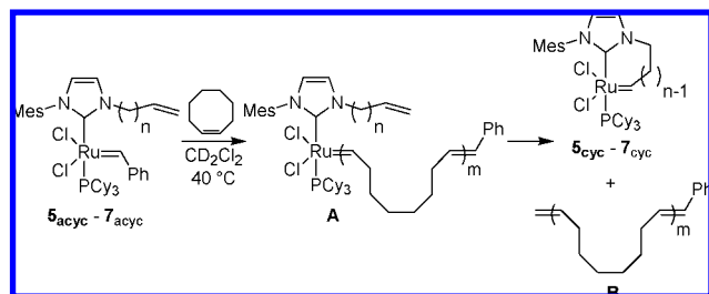
Scheme 4. Proposed Species Observable upon ROMP of COE Using Open Catalysts 5_{\text{acyc}}-7_{\text{acyc}}
