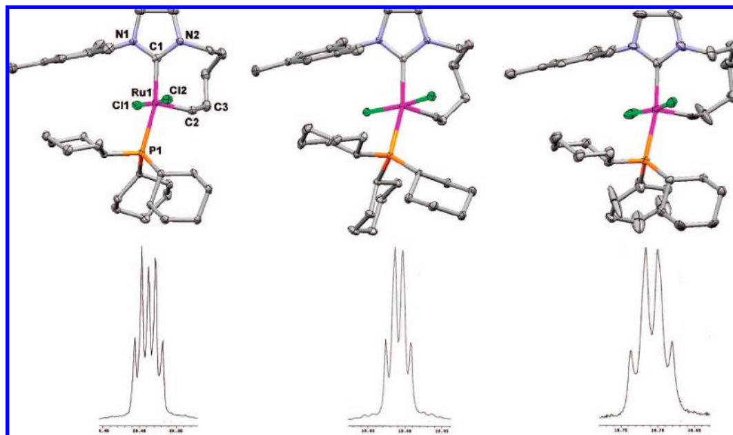
Figure 3. (Top) X-ray crystal structures of 5_{\text{cyc}}\cdot\text{H}_2 , 6_{\text{cyc}} , and 6_{\text{cyc}}\cdot\text{H}_2 . Solvent molecules and hydrogens have been removed for clarity. Ellipsoids are drawn at the 50% probability level. (Bottom) ^1\text{H} NMR spectra ( \text{C}_6\text{D}_6 ) of alkylidene proton of 5_{\text{cyc}}\cdot\text{H}_2 , 6_{\text{cyc}} , and 6_{\text{cyc}}\cdot\text{H}_2 .
