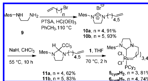
Scheme 3. Synthesis of “Saturated” Catalysts 5 cyc ·H 2 and 6 cyc ·H 2
