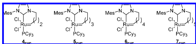
Figure 2. Cyclic Ru-alkylidene metathesis catalysts.
