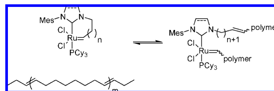
Scheme 5. Equilibration of Cyclic Catalyst and Linear PCOE
